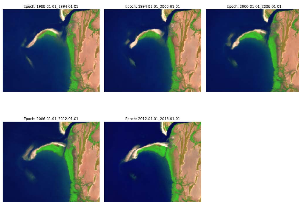
Figure 60. Geomorphic change at the Gilbert River estuary. Composite images of the mid-tide range for the area identified by the bounding box in Figure 35. The figure in the top left represents data composited between Jan 1988 and Jan 1994, increasing in 6-year increments from left to right, top to bottom. The bottom right figure represents data between Jan 2012 and the present.
