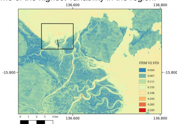
Figure 47. ITEM confidence layer for the McArthur River. The change detection highlighted in Figure 62 is represented by the black box. The transect represented in Figure 71 is shown in black.
