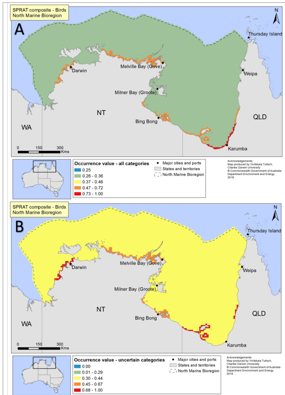
Figure 96. Composite species distribution maps for shorebirds (Red Knot, Curlew Sandpiper, Great Knot, Greater Sand-Plover, Lesser Sand-Plover, Eastern Curlew) derived from SPRAT rankings for (A) all SPRAT categories, and (B) for uncertain categories only (“may occur” and “likely”), which were summed for all 6 priority shorebird species, then re-scaled between 0 and 1. Scales between the two map types are not directly comparable.
