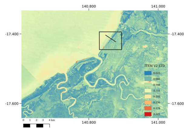
Figure 39. ITEM confidence layer for the Flinders River estuary. The transect represented in Figure 66 is shown in black. The bounding box highlights a region of significant coastal mangrove habitat dieback over the 2015/2016 Austral summer.
