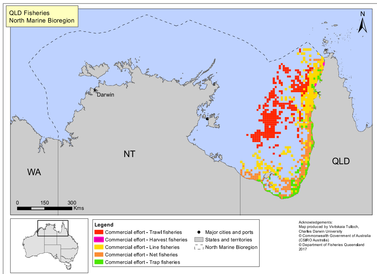
Figure 93. Cumulative fishing pressure map for QLD fisheries (Department of Agriculture and Fisheries), identifying spatial extent of fishery effort only, due to restrictions on data (low vessel numbers).
