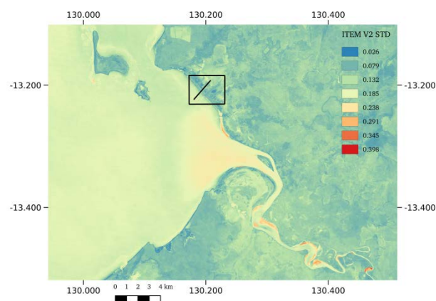
Figure 55. ITEM confidence layer for the Daly River estuary. Analyses for the region in black are not shown.
