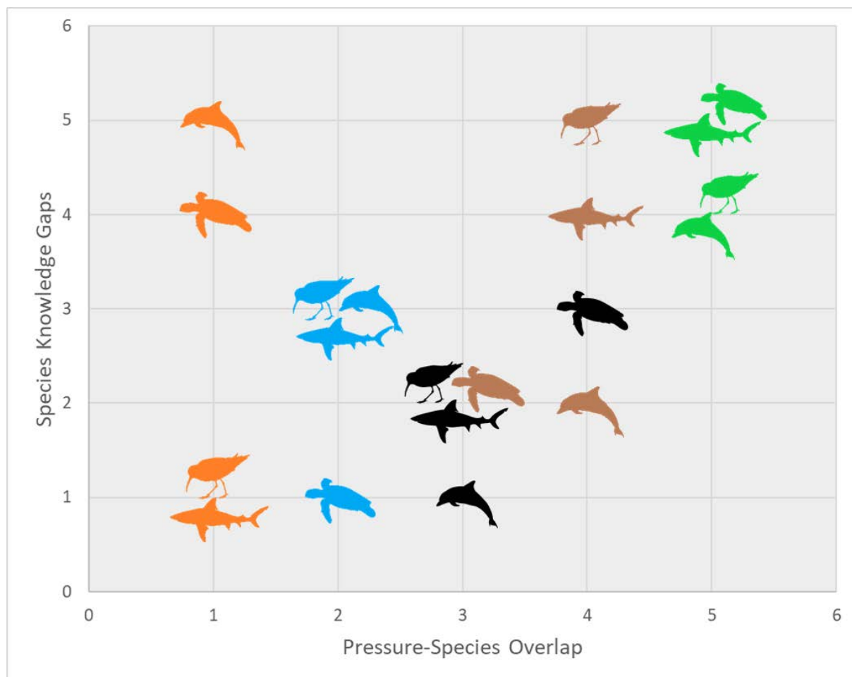
Figure 106. Species knowledge gap/pressure-species overlap plot for sharks and sawfishes, turtles, shorebirds and marine mammals for the five North Marine Bioregion sub-regions (Top End, black; Arnhem, blue; Western Gulf, brown; Southern Gulf, green; Cape York, orange; colours used here are not related to those in Table 19).
