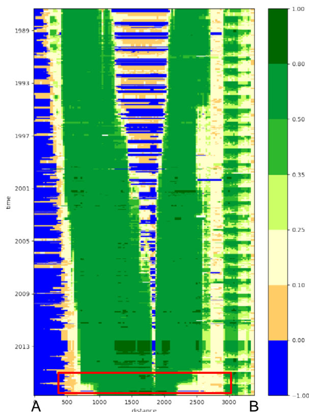
Figure 65. The transect in Figure 60 is represented on the x-axis of this Hovmoller plot, y-axis is time, colour is NDVI. The 2015–16 dieback event is highlighted in the red box.
