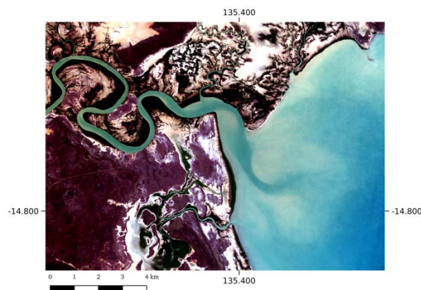
Figure 41. HOT composite image of the Roper River estuary.
