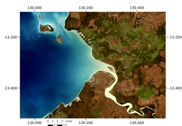
Figure 53. HOT composite image of the Daly River estuary.
