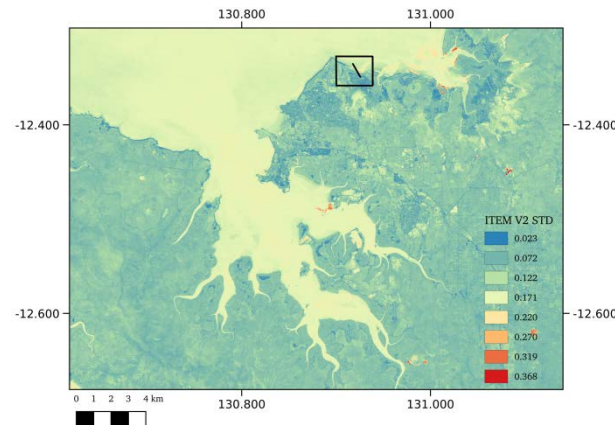
Figure 51. ITEM confidence layer for Darwin Harbour. Analyses for the regions in black are not shown.
