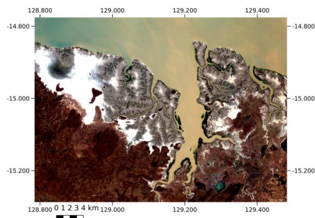
Figure 57. HOT composite image of the Keep River estuary.
