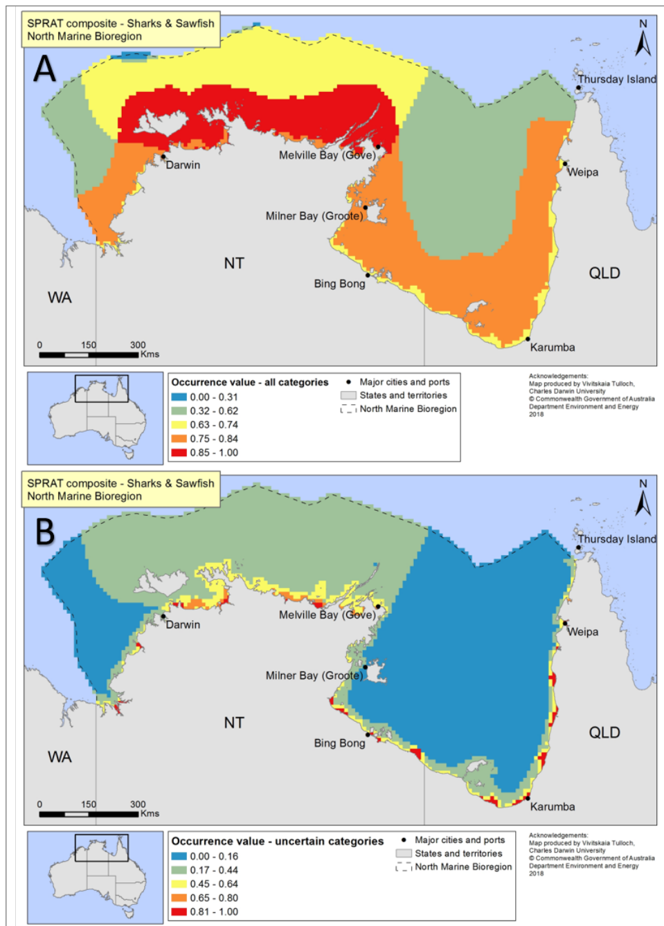
Figure 94. Composite species distribution maps for sharks and sawfishes (Northern River Shark, Speartooth Shark, Dwarf Sawfish, Largetooth Sawfish, Green Sawfish) from SPRAT rankings for (A) all SPRAT categories, and (B) for uncertain categories only (“may occur” and “likely”), which were summed for all 5 priority shark and sawfish species, then re-scaled between 0 and 1. Scales between the two map types are not directly comparable.
