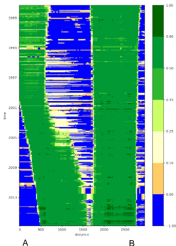
Figure 73. The Keep River estuary transect detailed in Figure 72 is represented on the x-axis of this NDVI Hovmoller plot.
